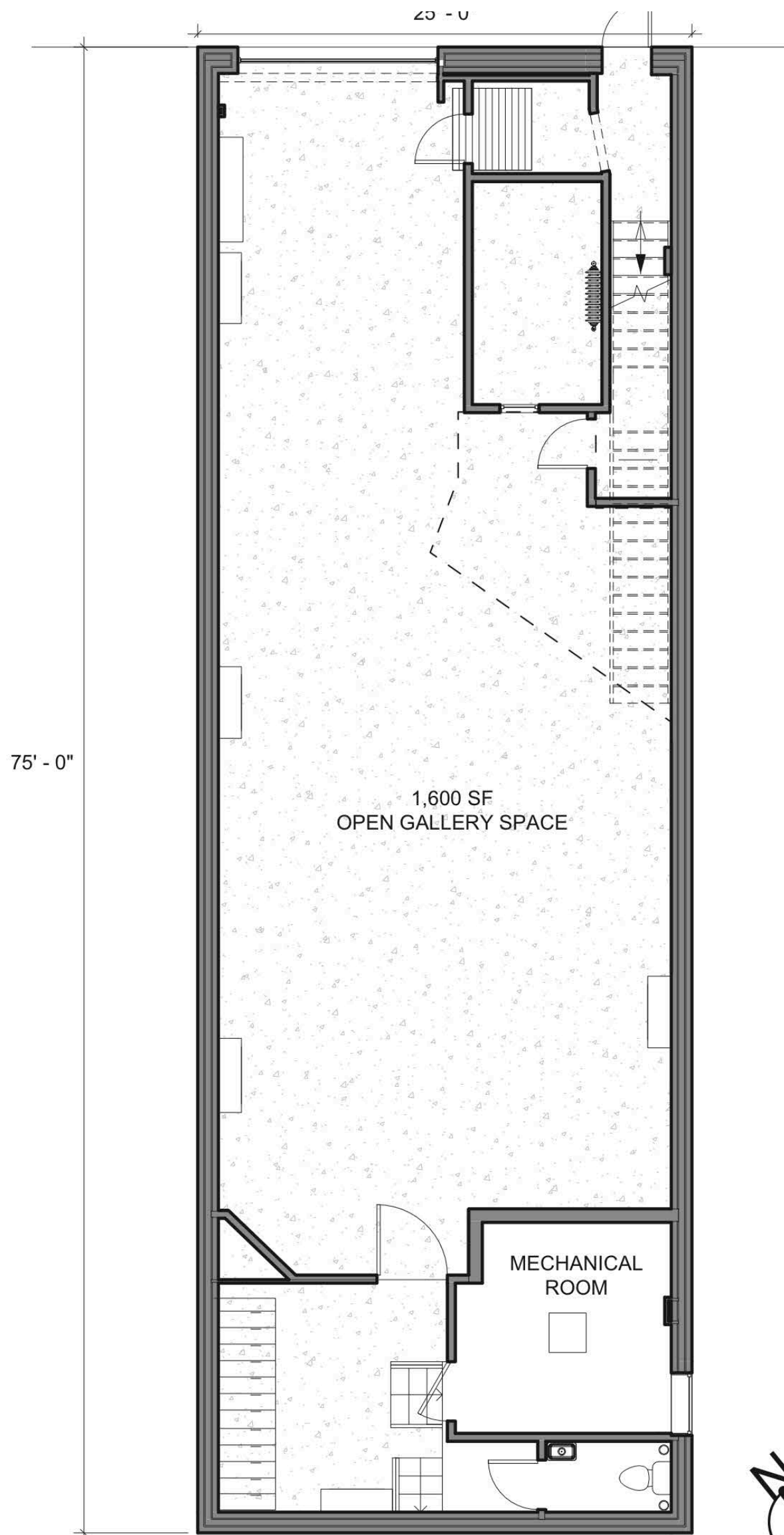
FIRST FLOOR
