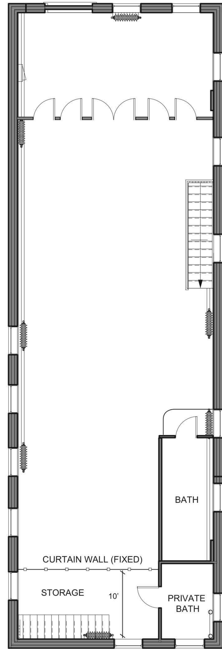
SECOND FLOOR
